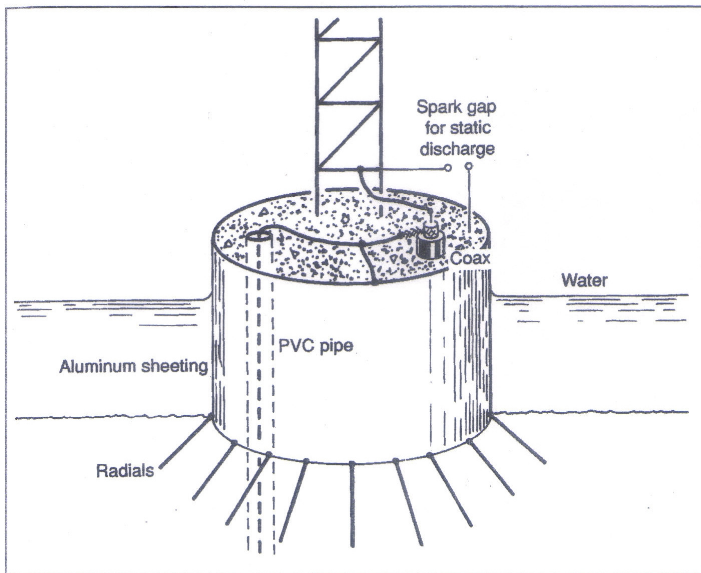
Fig. 1— Schematic of the base of PY3CEJ's 160 meter antenna system. The tower installed on the concrete base is 1/4 wavelength high and is used as the radiating part of the antenna. An identical length of wire is dropped into the sealed PVC pipe which goes 40 meters underground to form the image section of a half-wave dipole. Radials were added in the water to further improve signals.
